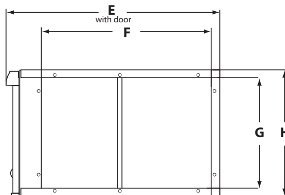
Inlet Side Return Duct Connection
