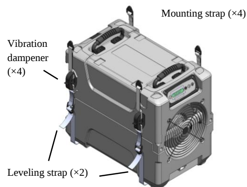
Fig. B: Suspension Straps
