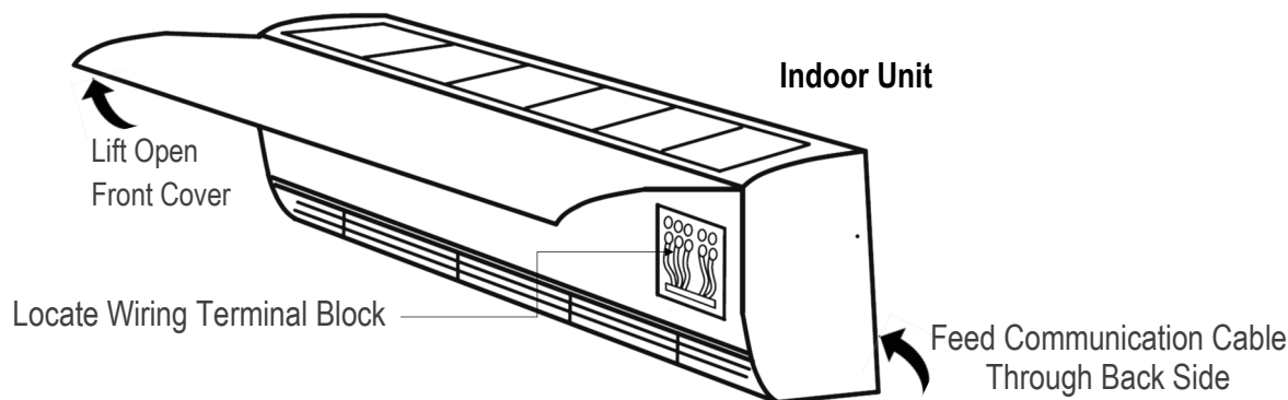
Fig. 4.4: Access Indoor Unit Wiring Block
