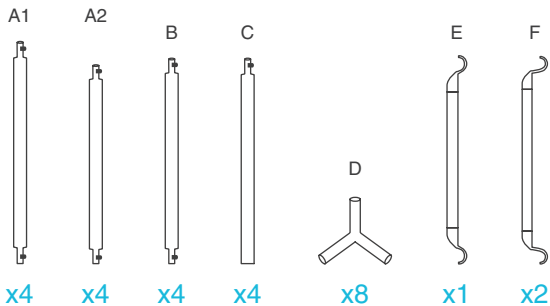
FRAME POLES
