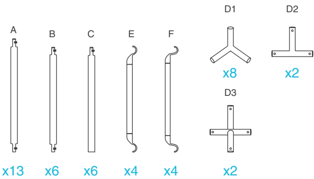
FRAME POLES
