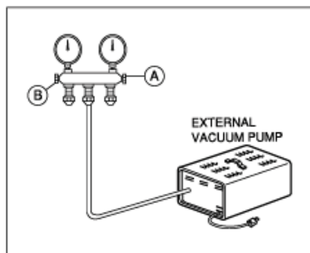
Figure 17A-Pulling Vacuum
