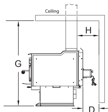
CORNER INSTALLATION CLEARANCE TO WALLS & CEILING
