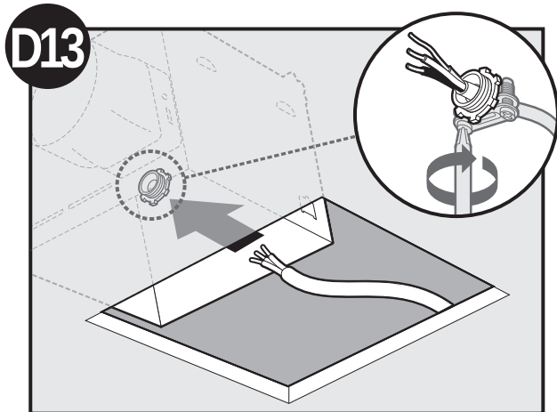
Pull wires through strain relief.
