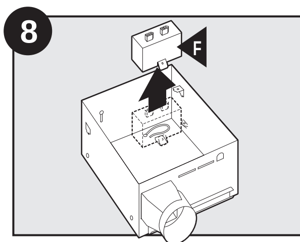
Remove the wiring cover.
