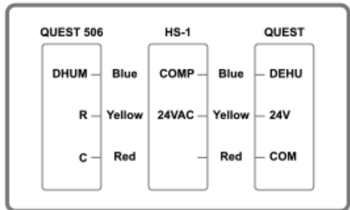
HS-1 wiring Diagram For Quest
