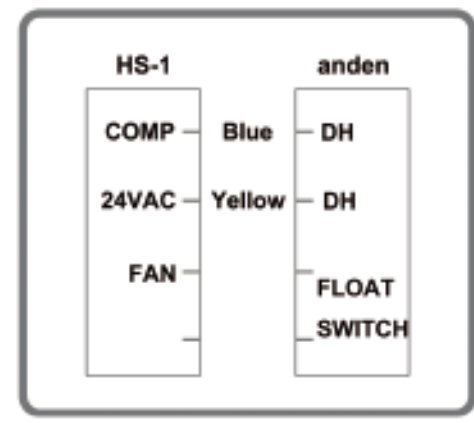
HS-1 Wiring Diagram For anden
