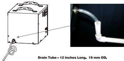
Drain Tube – 12 inches Long, 19 mm OD.
