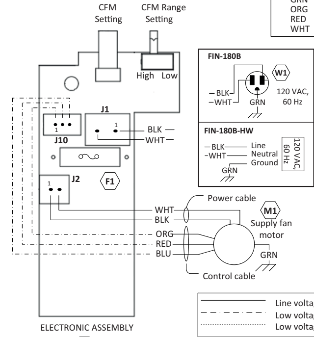
WIRING DIAGRAM
