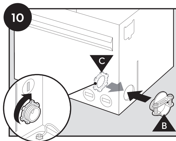
Insert the strain relief into the housing and secure with the washer.
