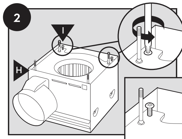
Loosen screws.
