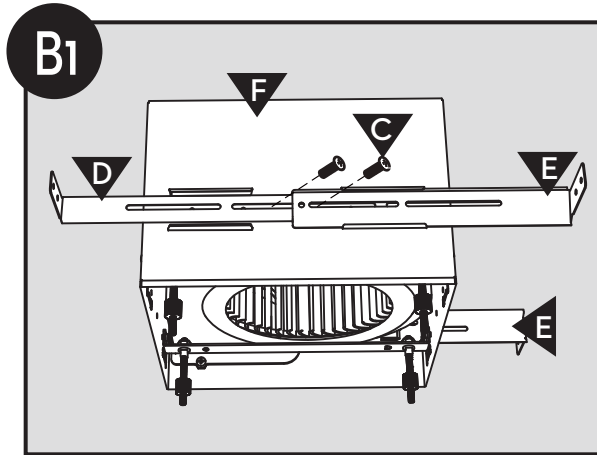
Slide the mounting rails into the side brackets and tighten with the machine screws.
