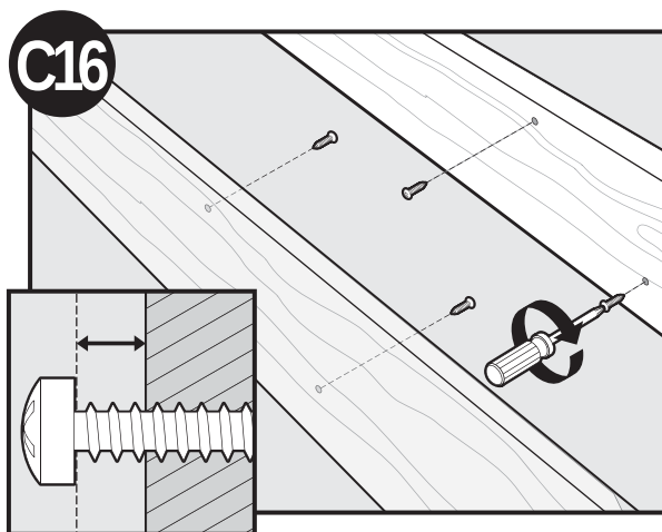
Insert screws, leaving space between the screw head and the joist. Screws are not provided.
