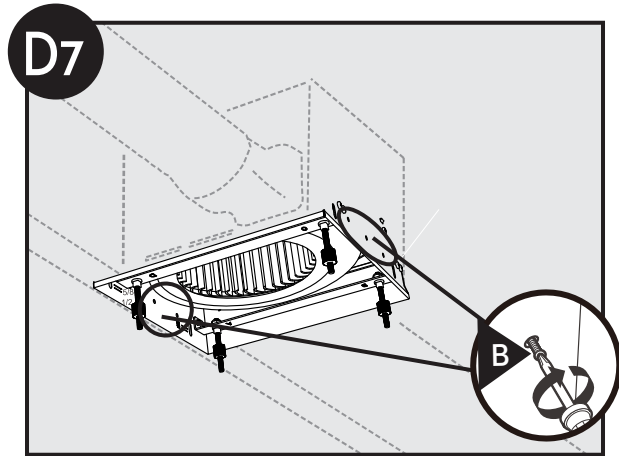
D7 Screw six (6) wood screws into joist or framing.
