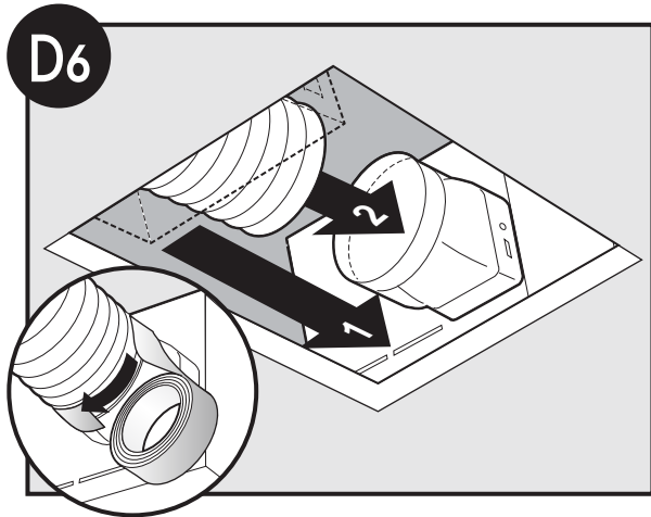
D6 Attach existing ducting to duct connector. Tape joints. If ducting does not fit securely, an adapter may need to be purchased.
