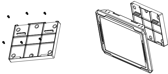
1. Mount the base panel on the wall with screws
