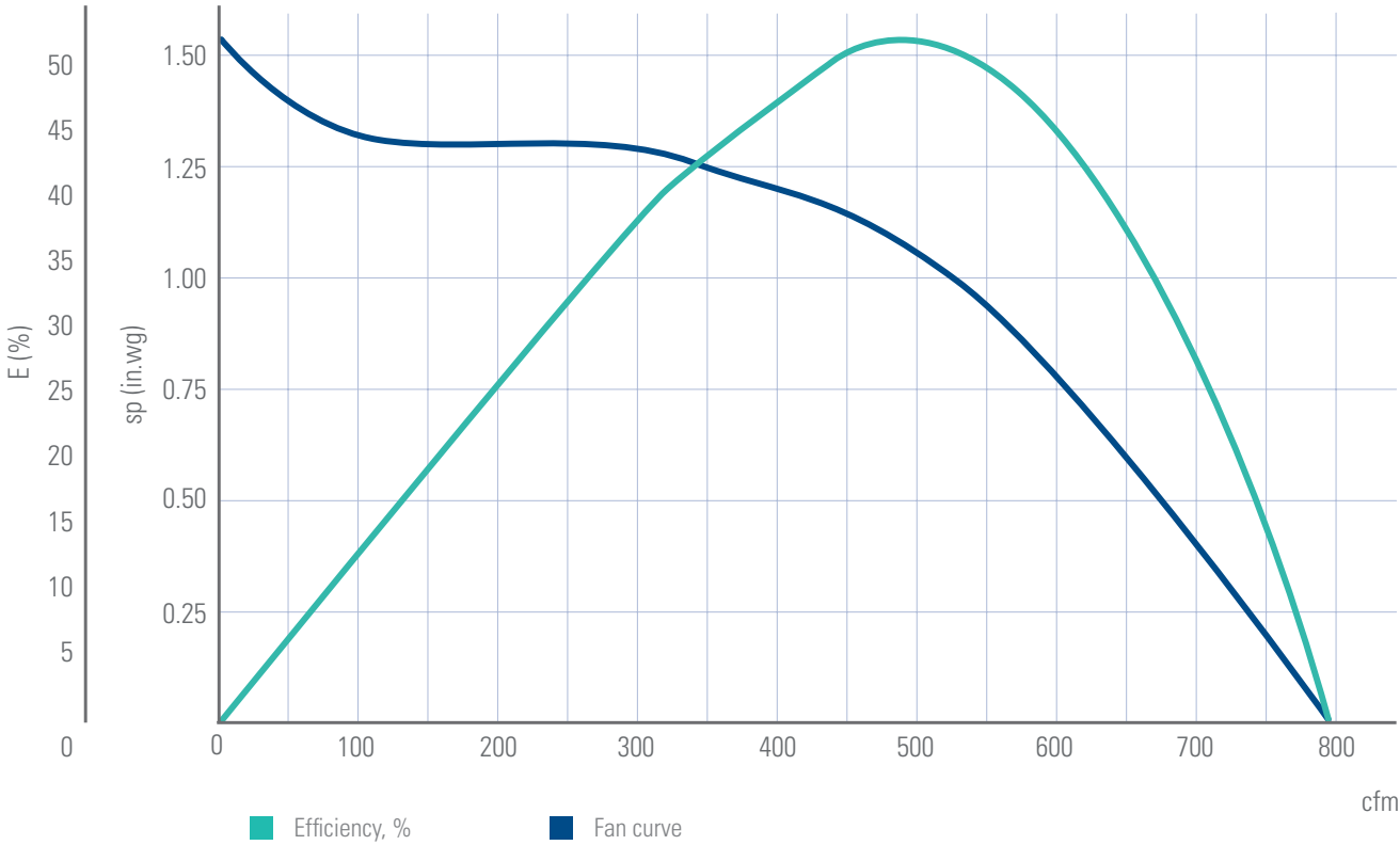
The graph represents airflow and efficiency for prioAir 8EC.
