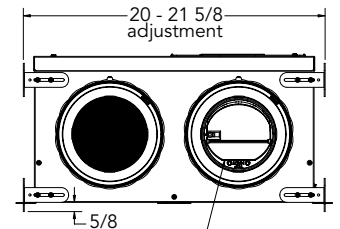
ORIENTABLE MAGNETIC BACKDRAFT DAMPER
