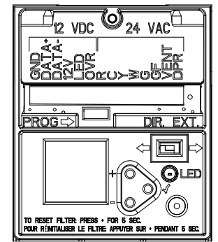
LCD SCREEN AND TERMINAL LOW VOLTAGE CONNECTIONS
