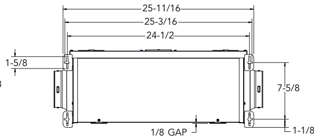
ORIENTABLE MAGNETIC BACKDRAFT DAMPER
