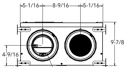
ORIENTABLE MAGNETIC BACKDRAFT DAMPER
